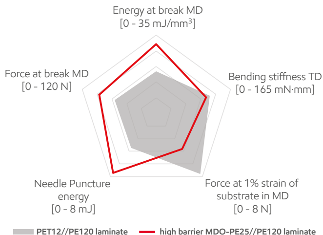
Graph 3 - Mechanical properties
